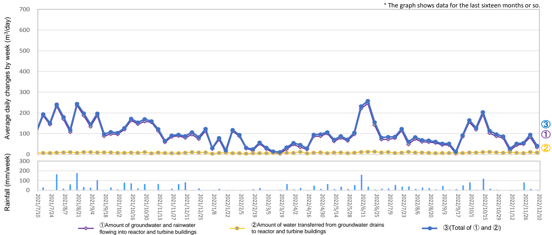
Amount of water transferred from groundwater drains to reactor and turbine buildings (From December 1, 2022 to December 7, 2022)
