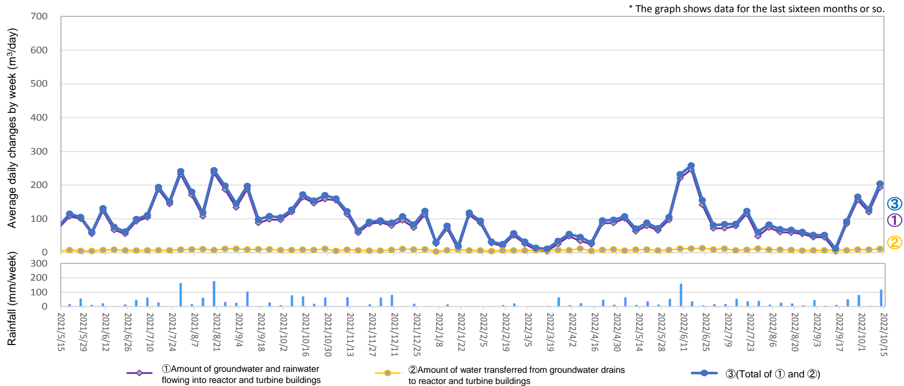
Amount of water transferred from groundwater drains to reactor and turbine buildings (From October 6, 2022 to October 12, 2022)
