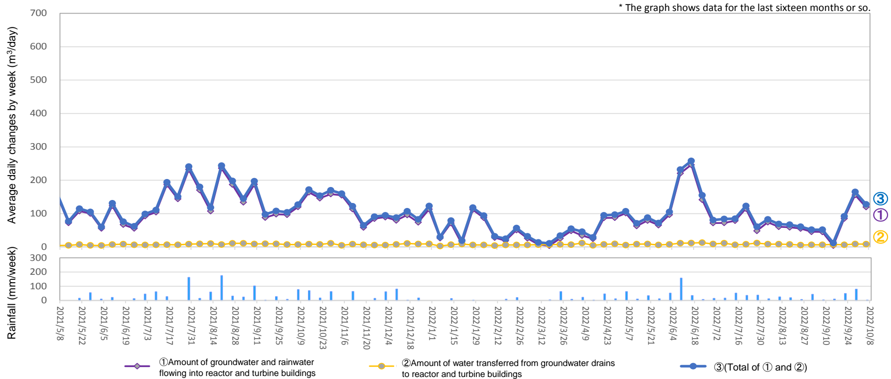
Amount of water transferred from groundwater drains to reactor and turbine buildings (From September 29, 2022 to October 5, 2022)
