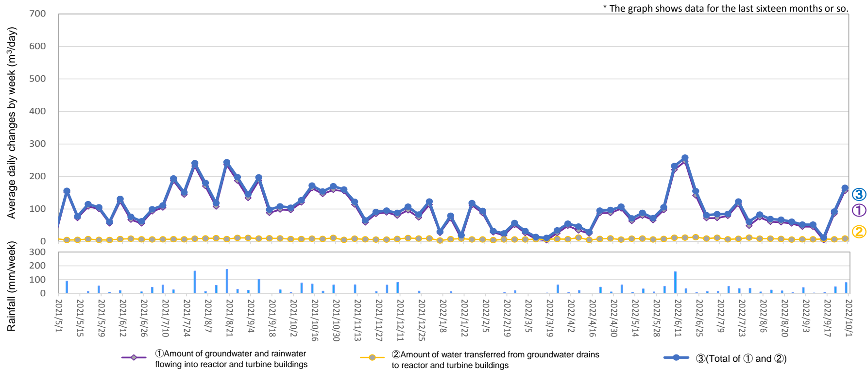
Amount of water transferred from groundwater drains to reactor and turbine buildings (From September 22, 2022 to September 28, 2022)
