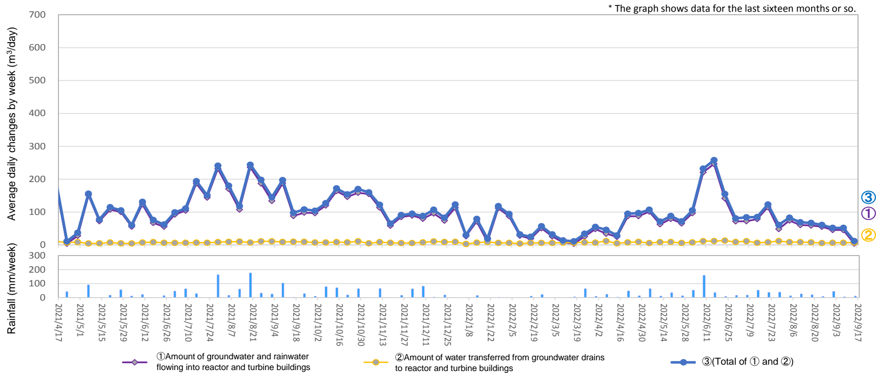
Amount of water transferred from groundwater drains to reactor and turbine buildings (From September 8, 2022 to September 14, 2022)
