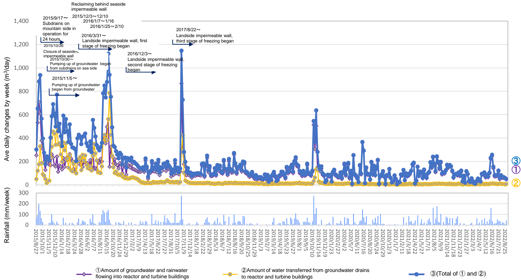
(Reference) Changes in the amount of water transferred from groundwater drains to reactor and turbine buildings
