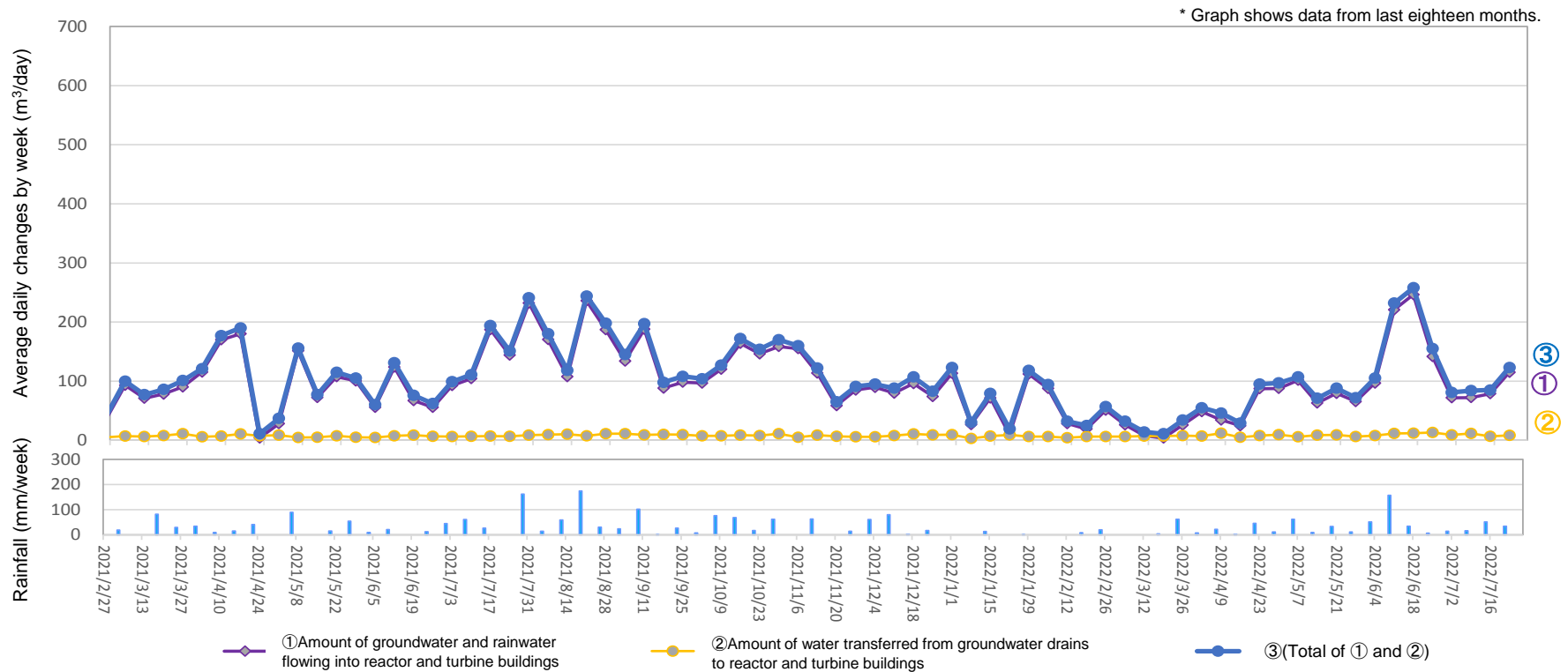
Amount of water transferred from groundwater drains to reactor and turbine buildings (From July 14, 2022 to July 20, 2022)
