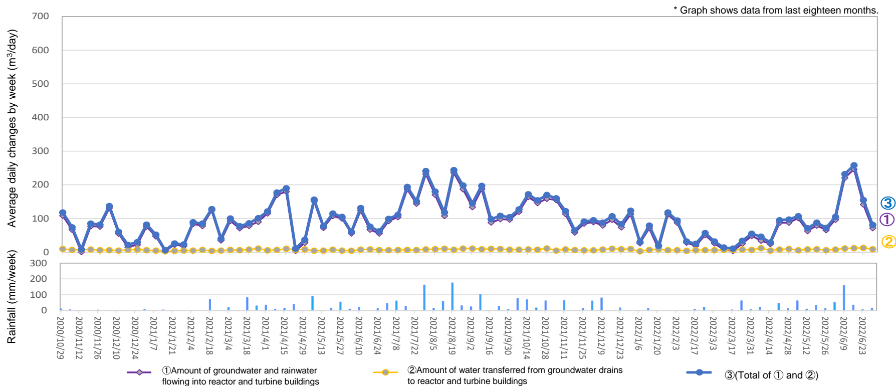
Amount of water transferred from groundwater drains to reactor and turbine buildings (From June 23, 2022 to June 29, 2022)
