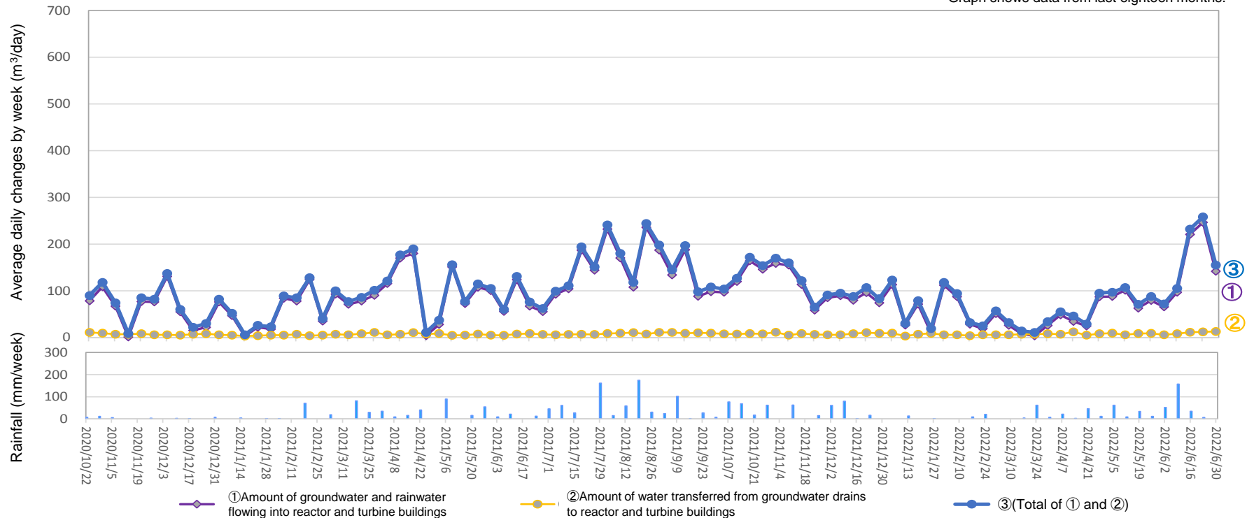
Amount of water transferred from groundwater drains to reactor and turbine buildings (From June 16, 2022 to June 22, 2022)
