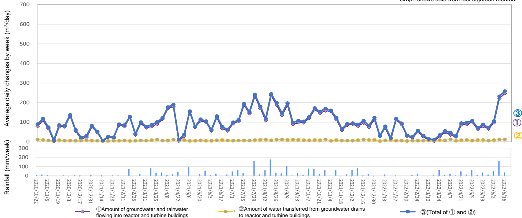
Amount of water transferred from groundwater drains to reactor and turbine buildings (From June 9, 2022 to June 15, 2022)
