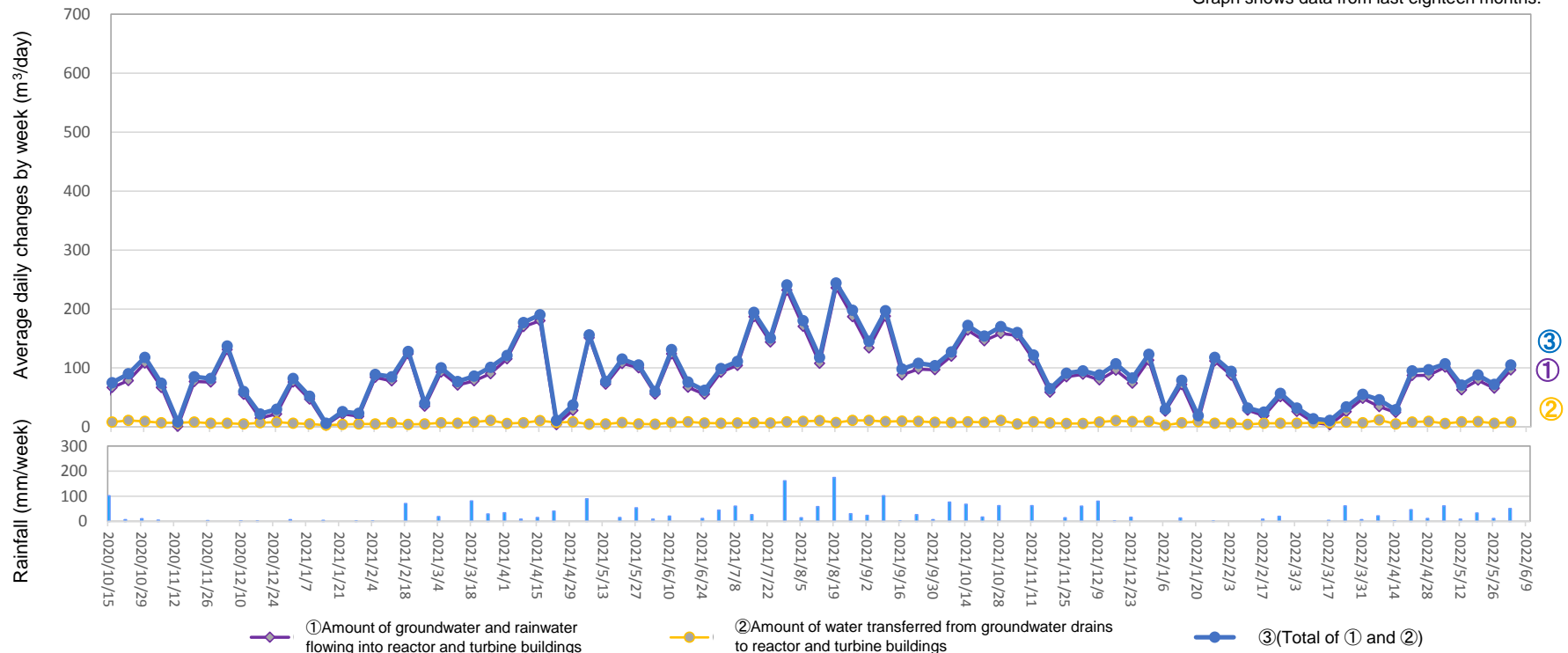
Amount of water transferred from groundwater drains to reactor and turbine buildings (From May 26, 2022 to June 1, 2022)
