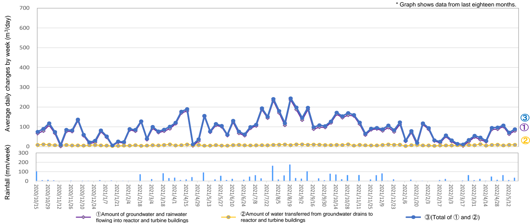
Amount of water transferred from groundwater drains to reactor and turbine buildings (From May 12, 2022 to May 18, 2022)
