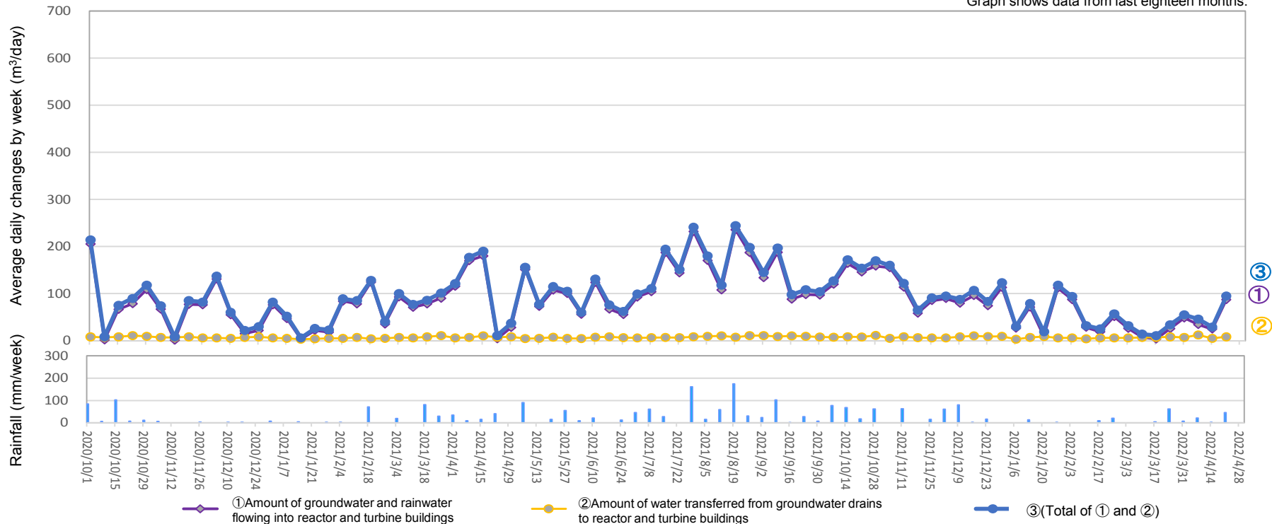
Amount of water transferred from groundwater drains to reactor and turbine buildings (From April 14, 2022 to April 20, 2022)
