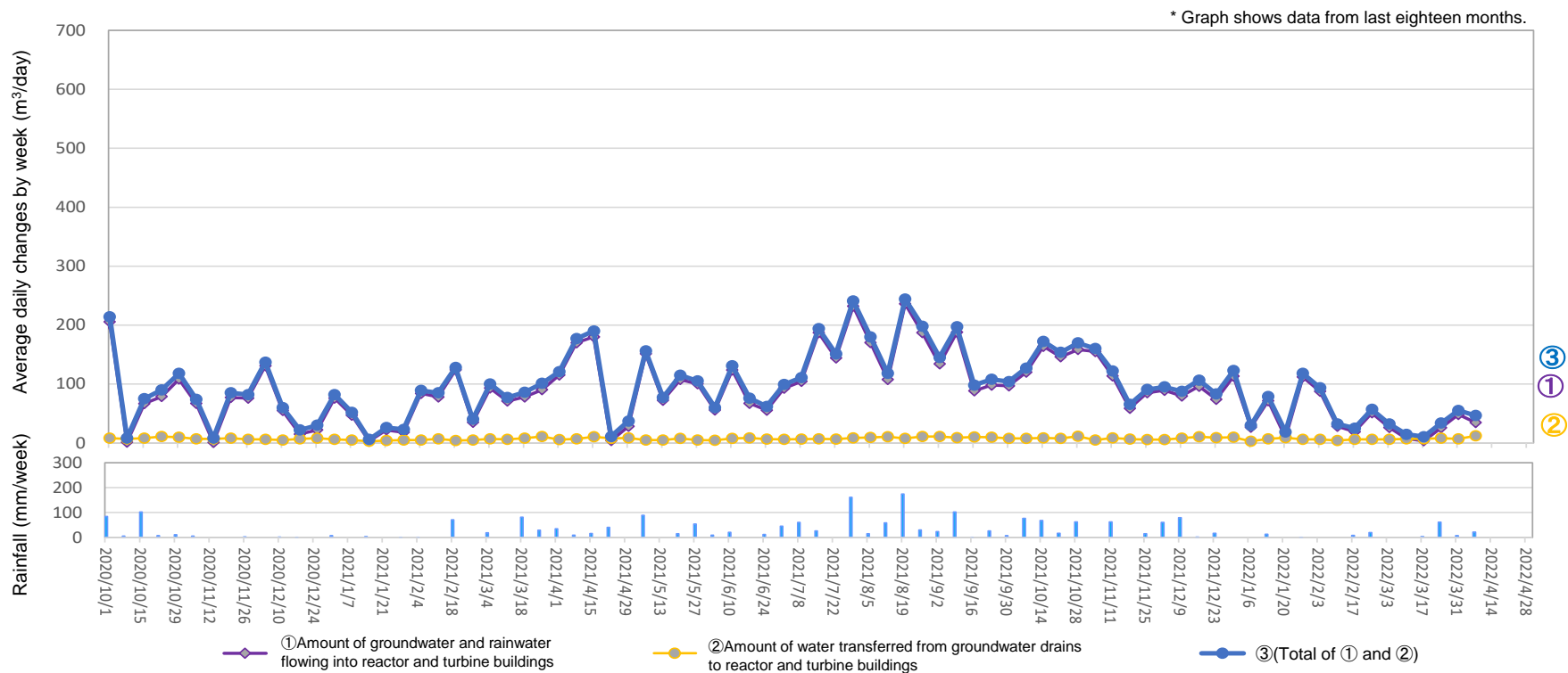
Amount of water transferred from groundwater drains to reactor and turbine buildings (From March 31, 2022 to April 6, 2022)
