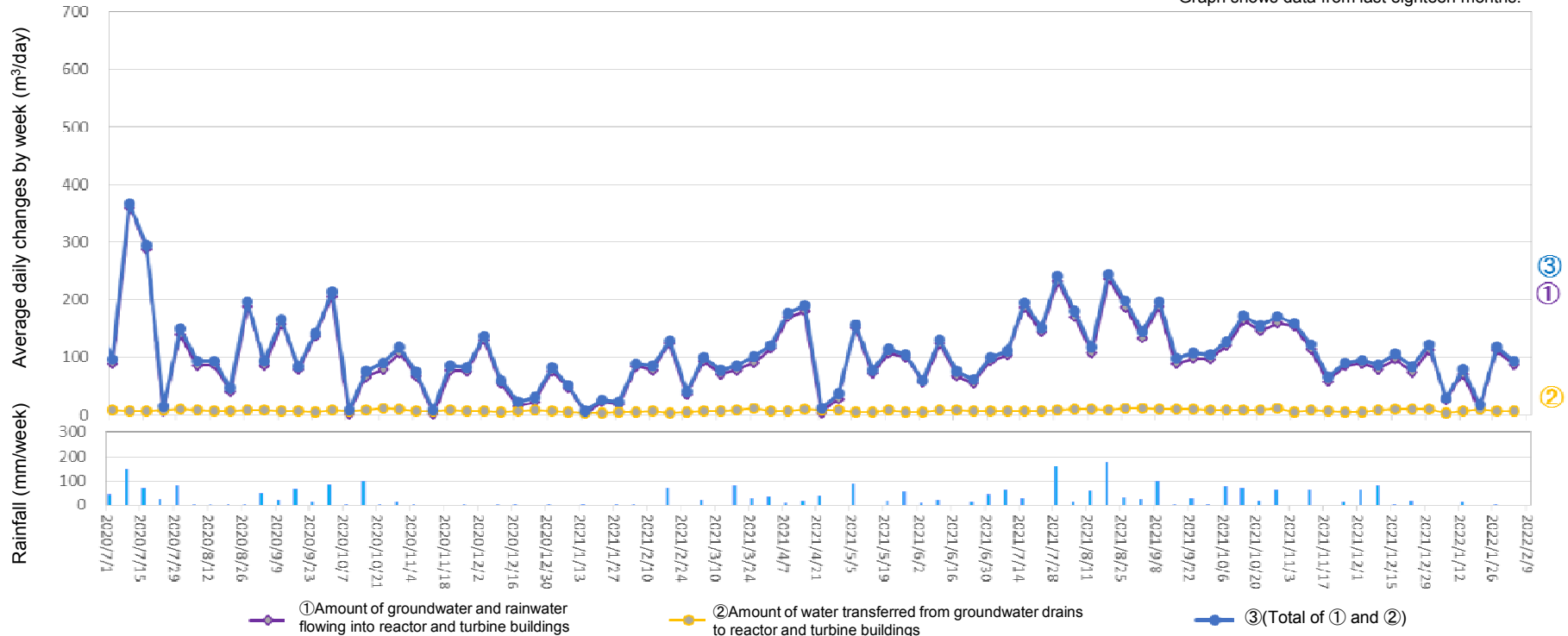
Amount of water transferred from groundwater drains to reactor and turbine buildings (From January 27, 2022 to February 2, 2022)
