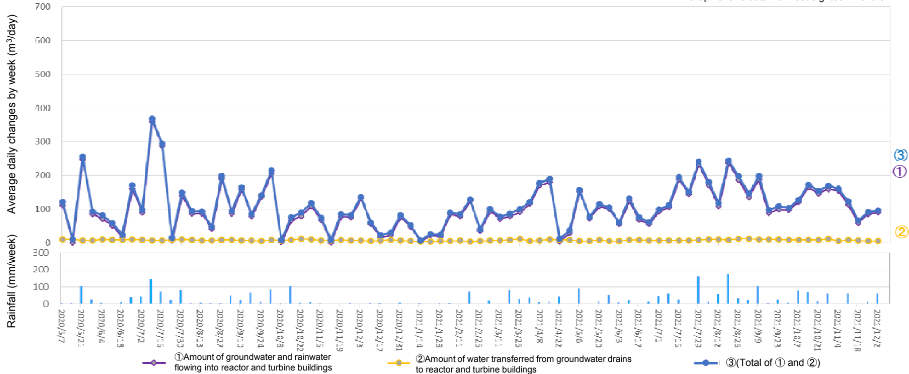
Amount of water transferred from groundwater drains to reactor and turbine buildings (From November 25, 2021 to December 1, 2021)
