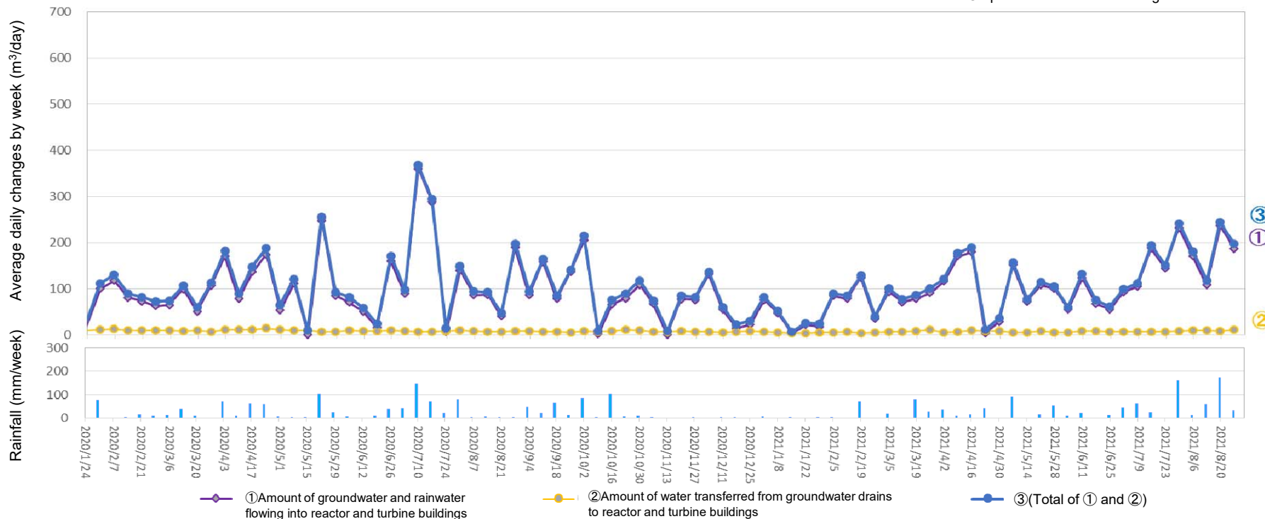
Amount of water transferred from groundwater drains to reactor and turbine buildings (From August 19, 2021 to August 25, 2021)
