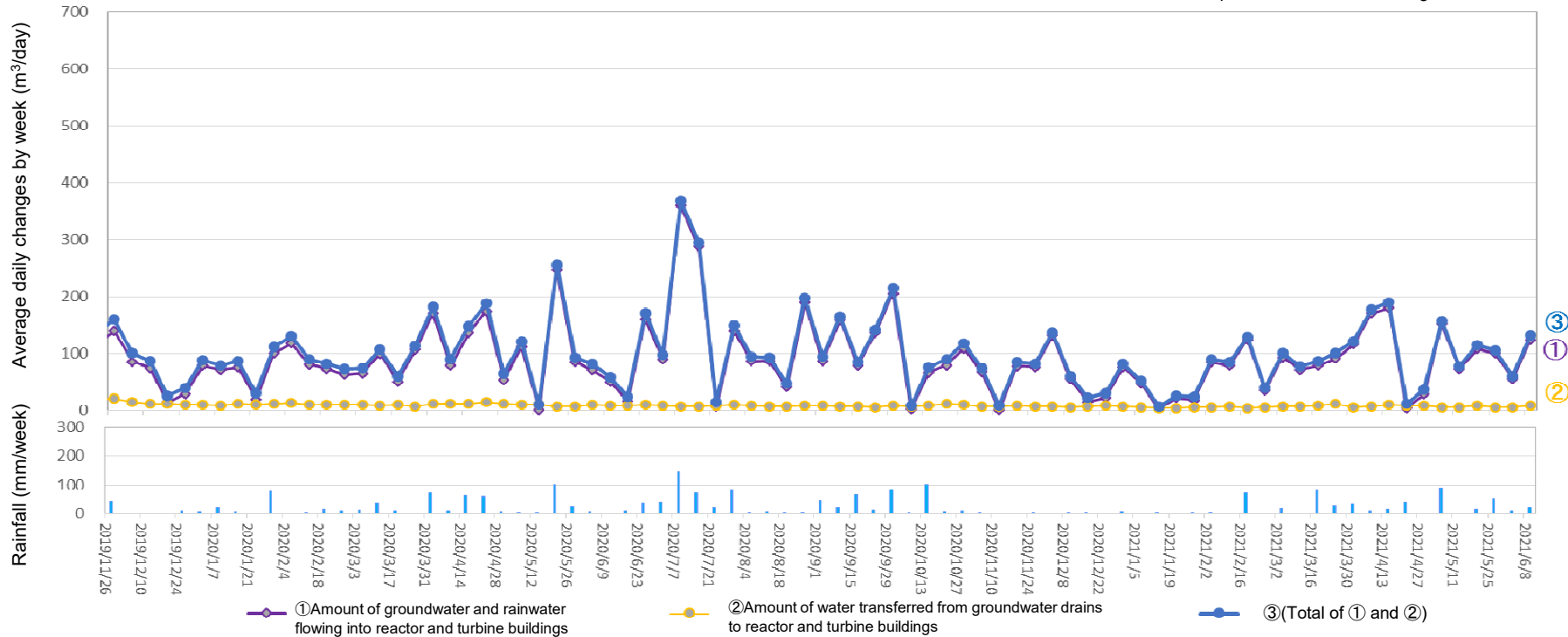
Amount of water transferred from groundwater drains to reactor and turbine buildings (From June 3, 2021 to June 9, 2021)
