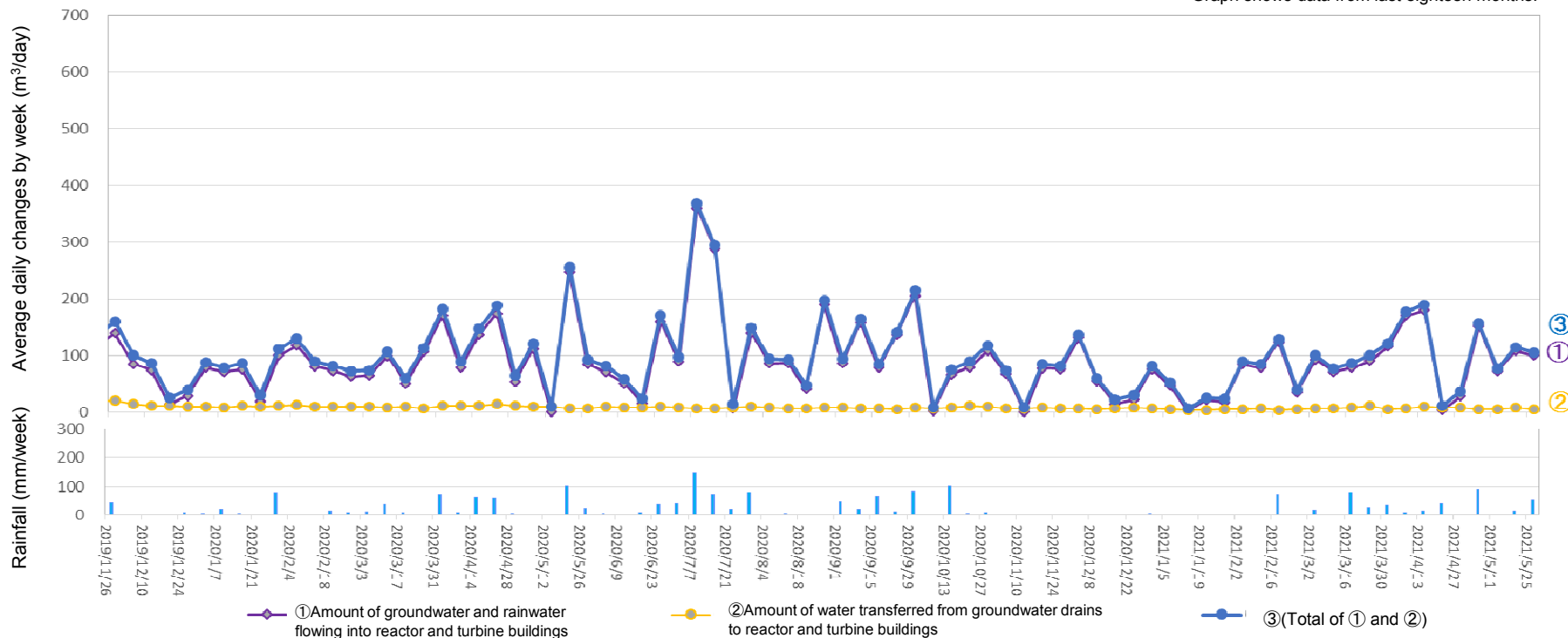
Amount of water transferred from groundwater drains to reactor and turbine buildings (From May 20, 2021 to May 26, 2021)
