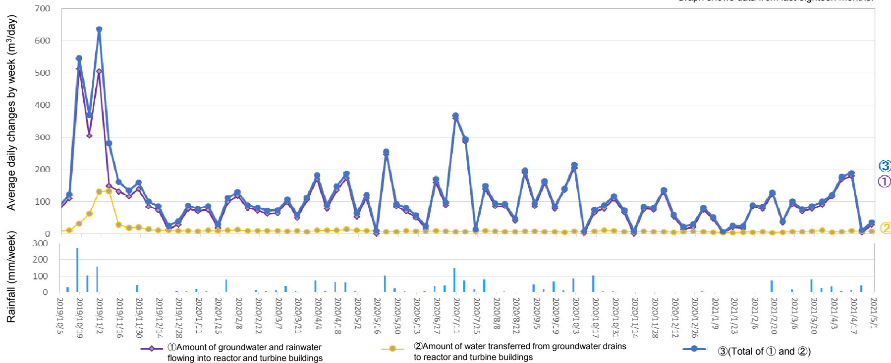
Amount of water transferred from groundwater drains to reactor and turbine buildings (From April 22, 2021 to April 28, 2021)
