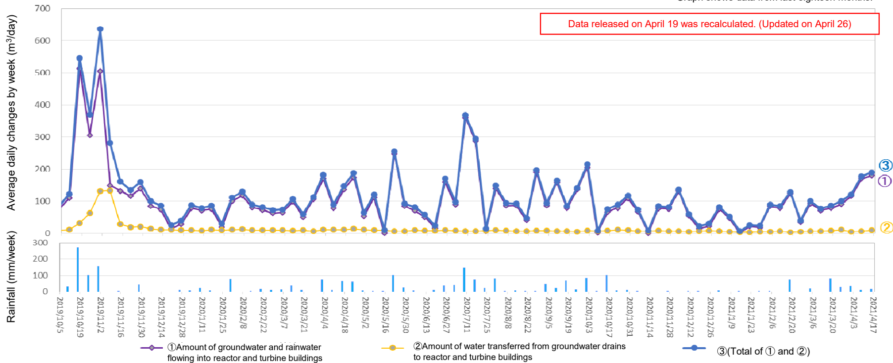
Amount of water transferred from groundwater drains to reactor and turbine buildings (From April 8, 2021 to April 14, 2021)
