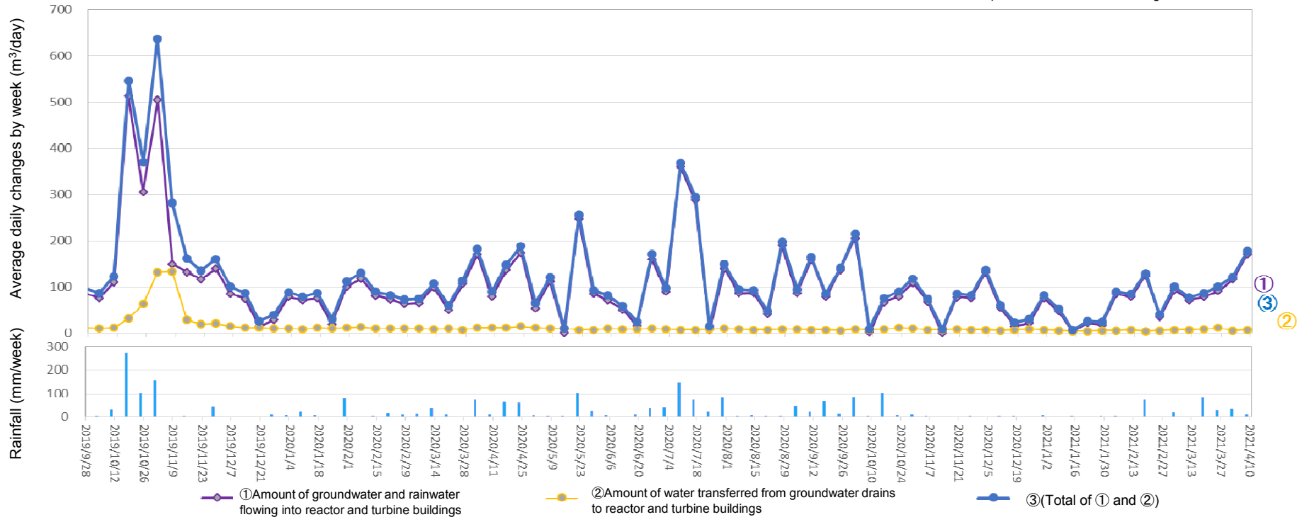
Amount of water transferred from groundwater drains to reactor and turbine buildings (From April 1, 2021 to April 7, 2021)
