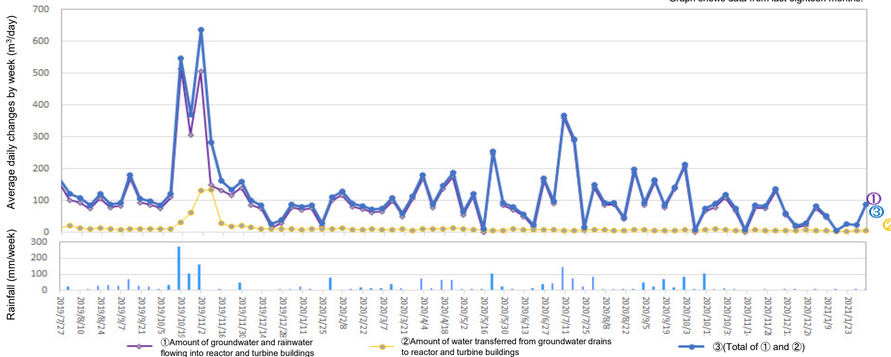
Amount of water transferred from groundwater drains to reactor and turbine buildings (From Jan 28, 2021 to Feb 3, 2021)
