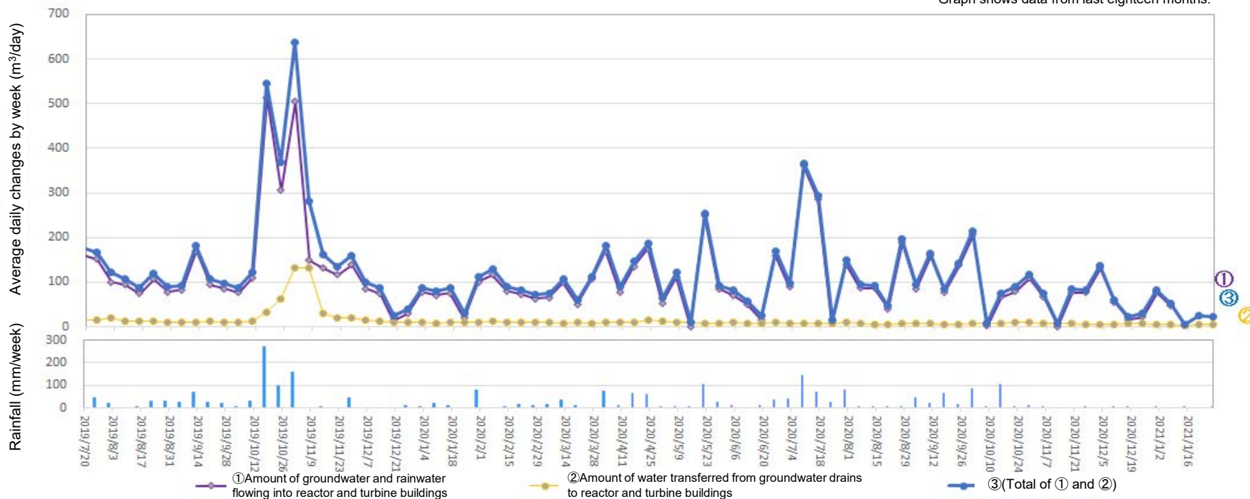
Amount of water transferred from groundwater drains to reactor and turbine buildings (From Jan 21, 2021 to Jan 27, 2021)
