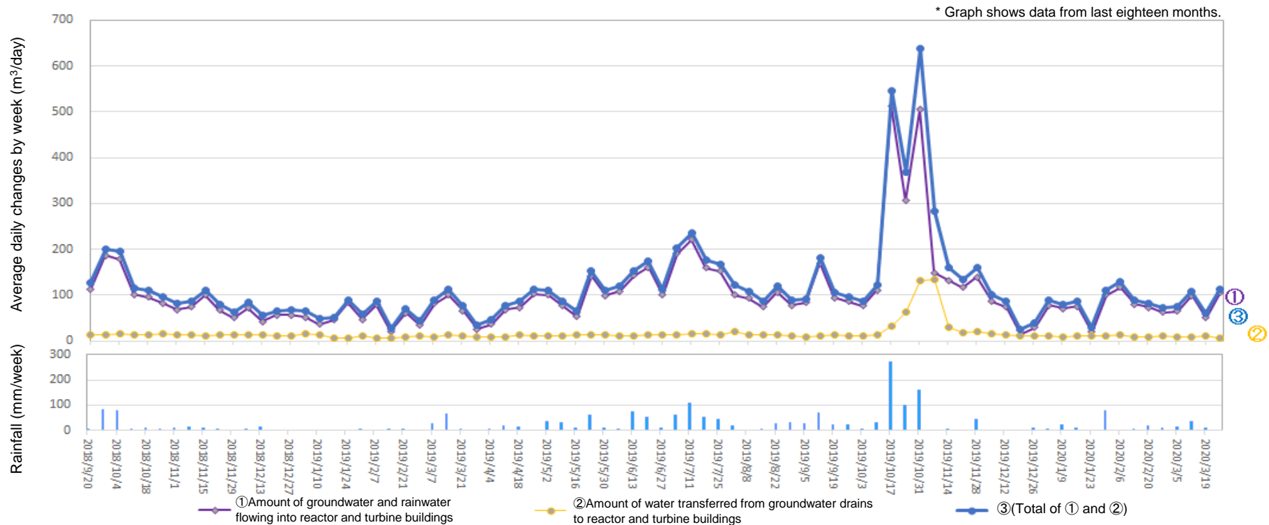
Amount of water transferred from groundwater drains to reactor and turbine buildings (From Mar 19, 2020 to Mar 25, 2020)
