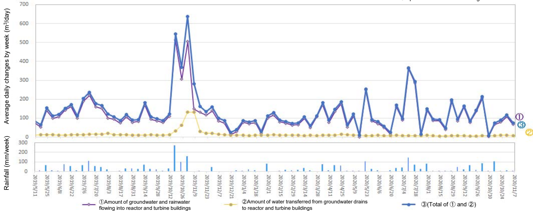
Amount of water transferred from groundwater drains to reactor and turbine buildings (From Oct 29, 2020 to Nov 4, 2020)
