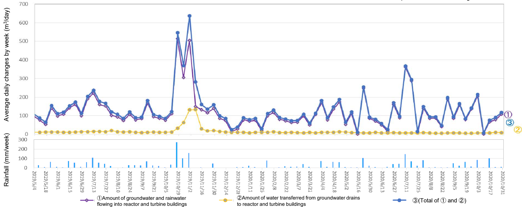
Amount of water transferred from groundwater drains to reactor and turbine buildings (From Oct 22, 2020 to Oct 28, 2020)
