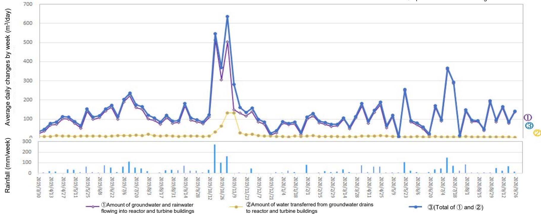
Amount of water transferred from groundwater drains to reactor and turbine buildings (From Sept 17, 2020 to Sept 23, 2020)
