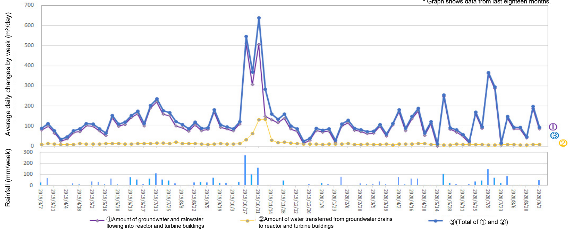
Amount of water transferred from groundwater drains to reactor and turbine buildings (From Aug 27, 2020 to Sept 2, 2020)
