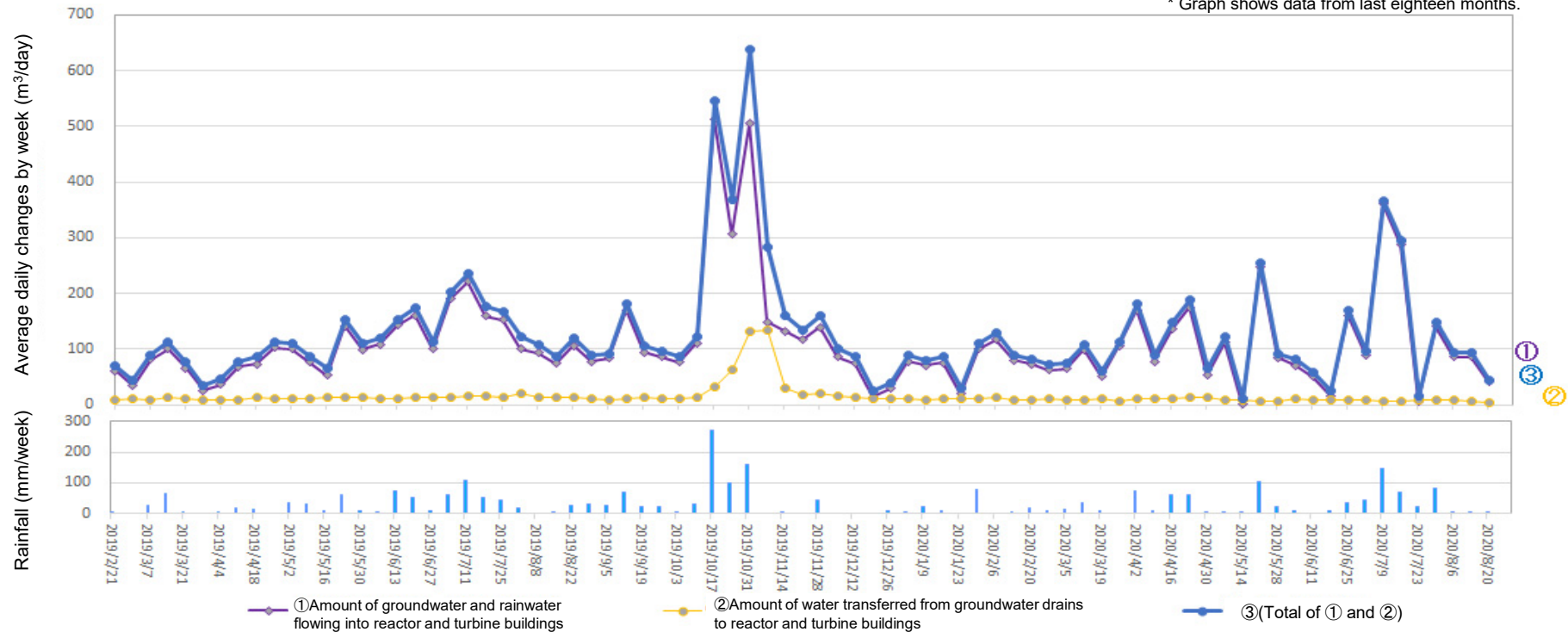
Amount of water transferred from groundwater drains to reactor and turbine buildings (From Aug 13, 2020 to Aug 19, 2020)
