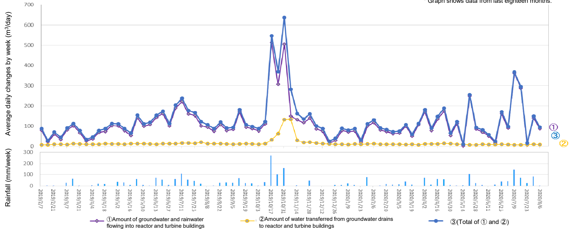
Amount of water transferred from groundwater drains to reactor and turbine buildings (From Jul 30, 2020 to Aug 5, 2020)
