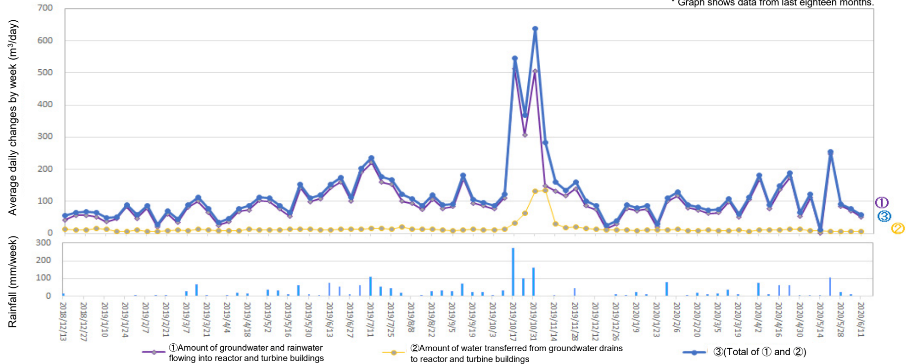
Amount of water transferred from groundwater drains to reactor and turbine buildings (From Jun 4, 2020 to Jun 10, 2020)
