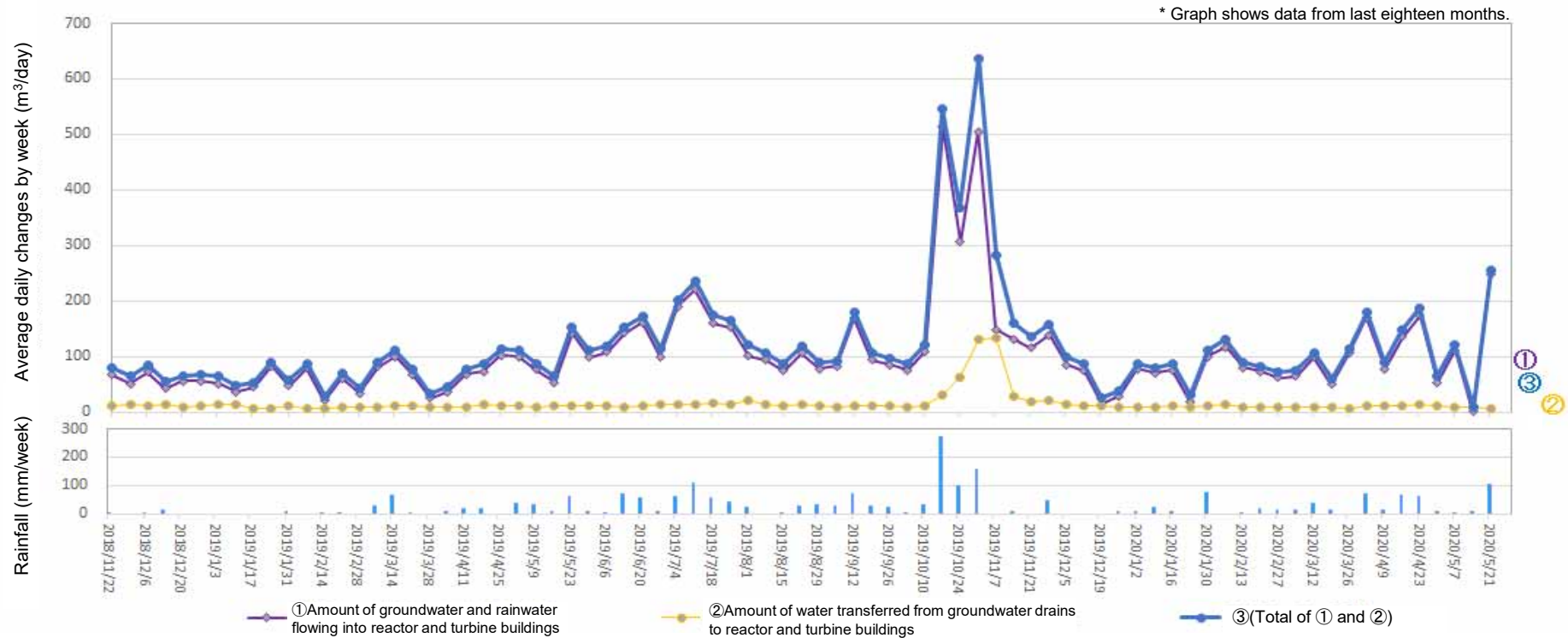
Amount of water transferred from groundwater drains to reactor and turbine buildings (From May 14, 2020 to May 20, 2020)
