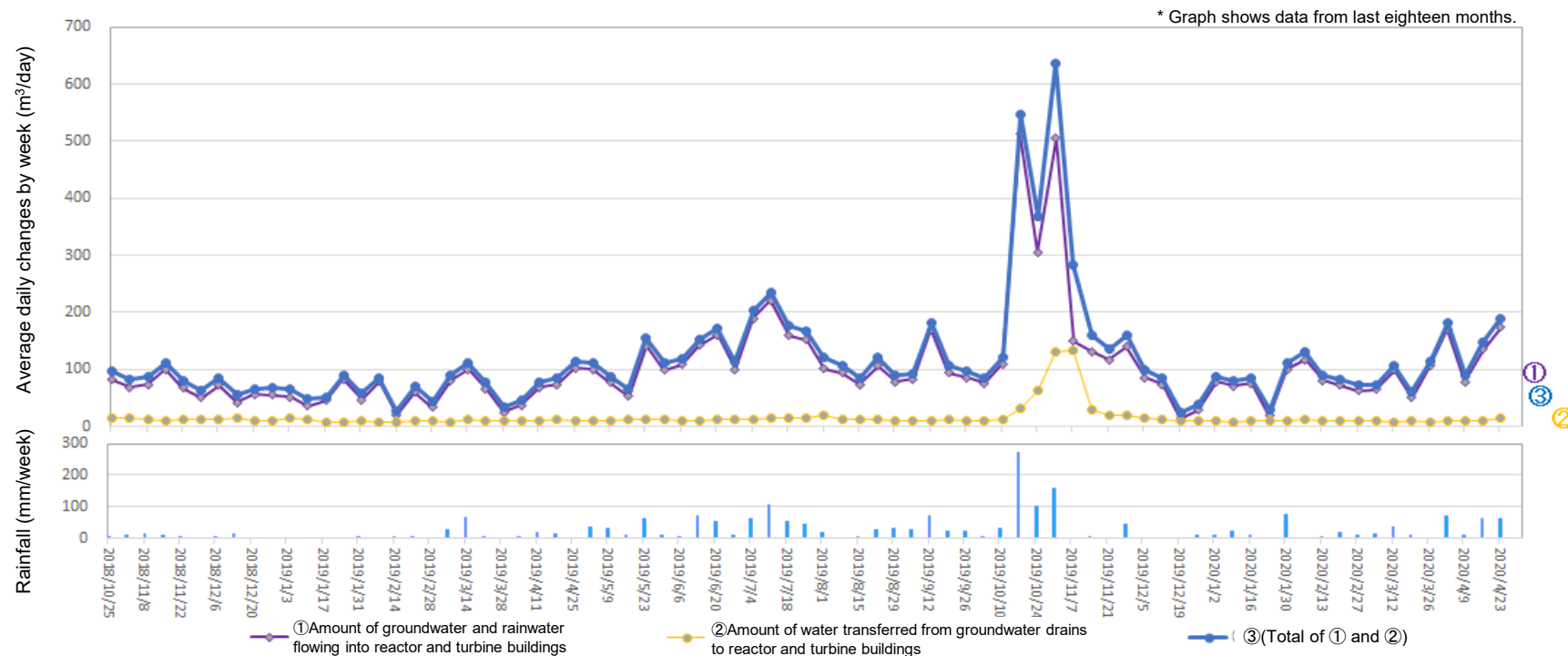
Amount of water transferred from groundwater drains to reactor and turbine buildings (From Apr 16, 2020 to Apr 22, 2020)
