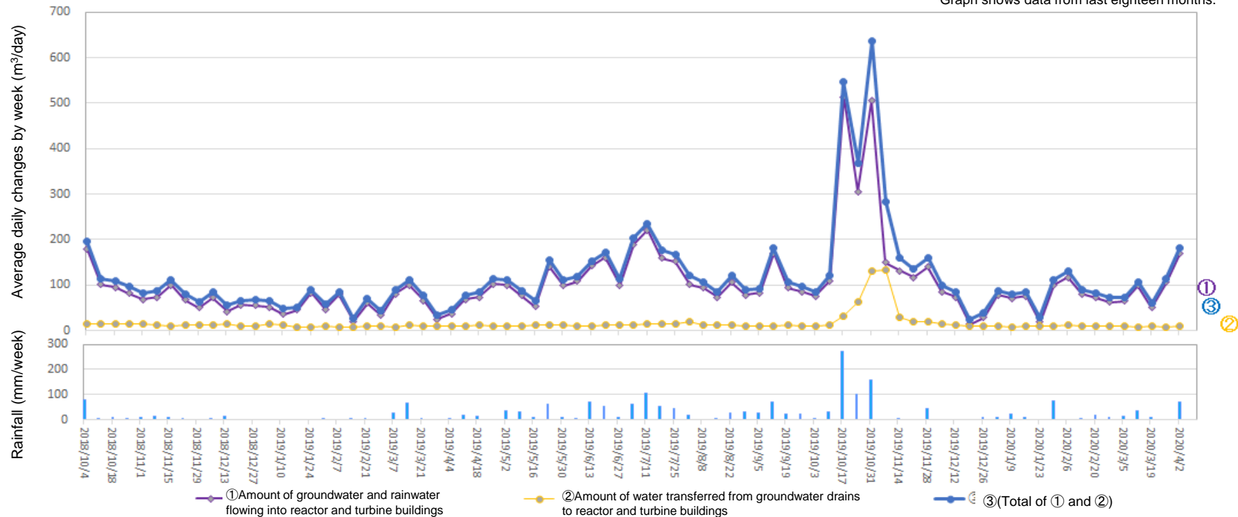
Amount of water transferred from groundwater drains to reactor and turbine buildings (From Mar 26, 2020 to Apr 1, 2020)
