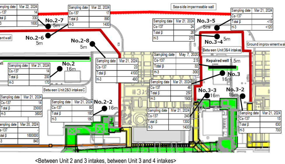
Figure 4: Groundwater concentration on the Turbine Building east side
