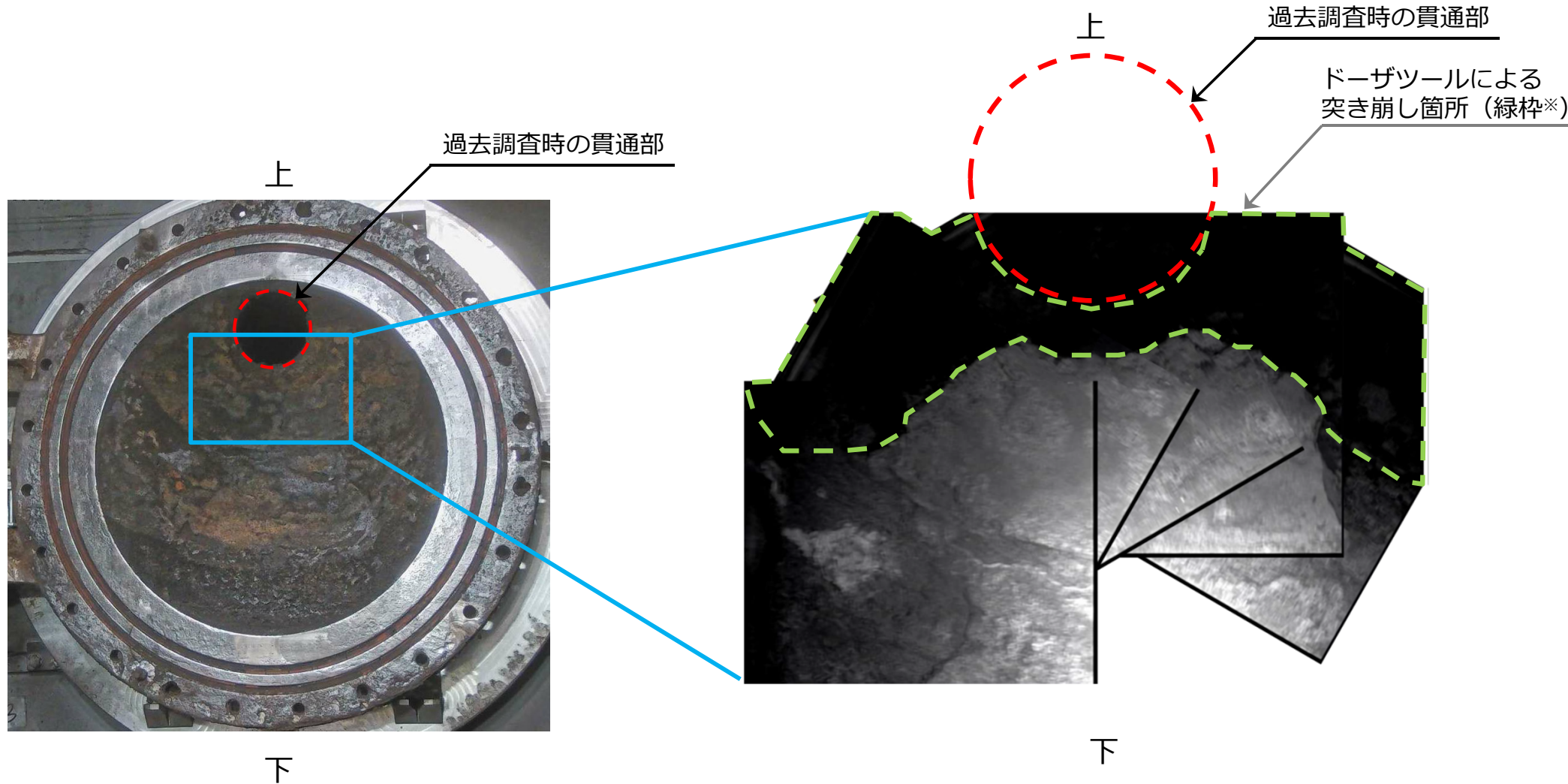
X-6ペネ外観
