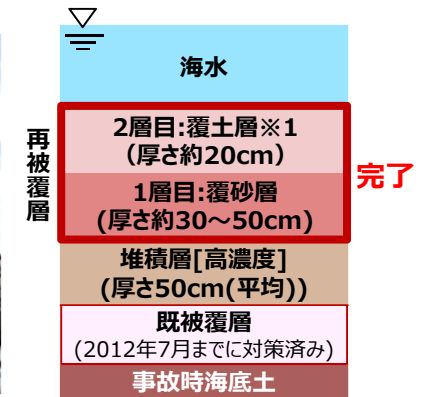
図6.層構成詳細
