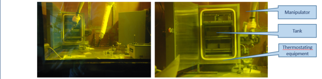
Installation of the prepared thermostatic equipment units inside the hot cell
