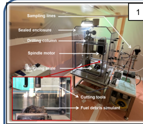
1. Coatings have been implemented on FD simulants (2) before core-boring in a specific airtight cell (1). Airborne particles production is monitored in order to assess the efficiency of the coating in terms of dust resuspension suppression (3)
