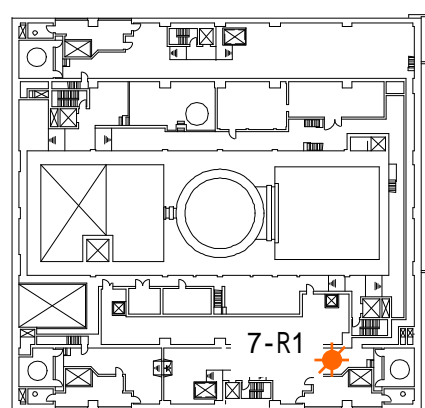
3階(T.M.S.L.+23.5m)
