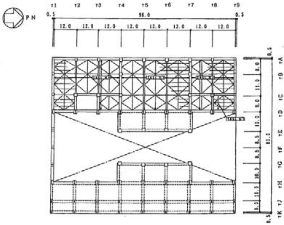
図-3.3.15 3階 (T.M.S.L. 30.9m)
