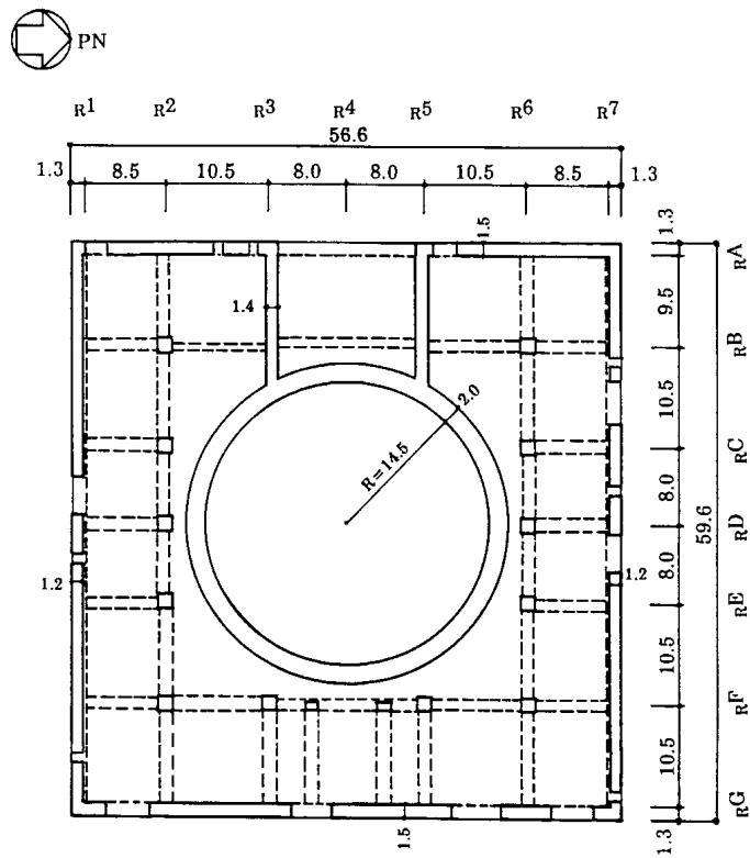
图-3.3.5 1階 (T.M.S.L. 12.3m)
